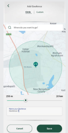
Geofencing
